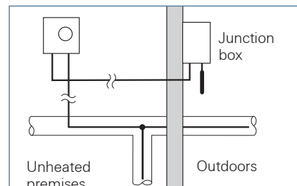
Always place the sensor in the coldest part of the installation
